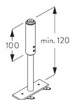
SG 6105 Hanger with plate
