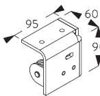
SG 8609 Pulley bracket ceiling right
