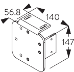
SG 8606 Roller bracket ceiling left
